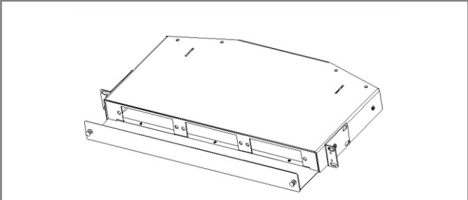
1 RU Fiber Management Panel with Sliding Drawer (17"W x 1.7"H x 12"D)
