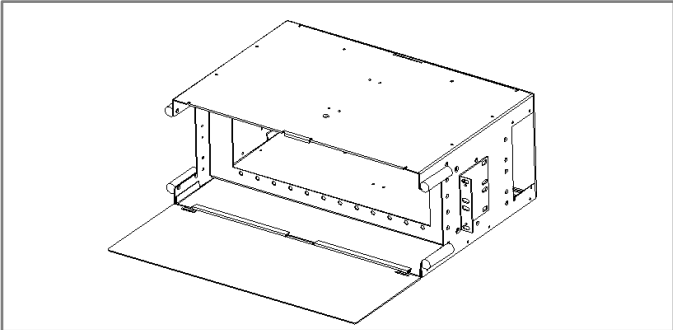
4RU Fiber Management Panel (17"W x 7"H x 12"D)
