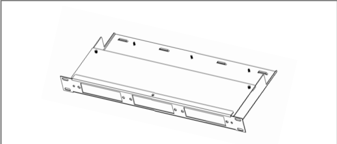
1 RU Fiber Management Panel (17"W x 1.7"H x 8"D)
