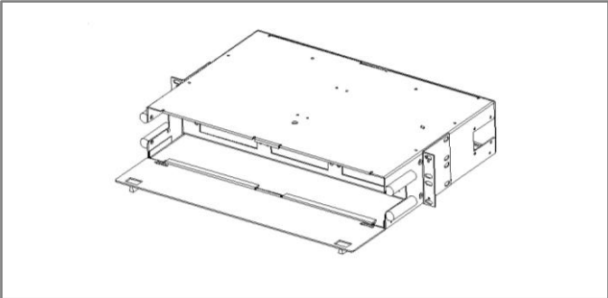
2RU Fiber Management Panel (17"W x 3.5"H x 12"D)
