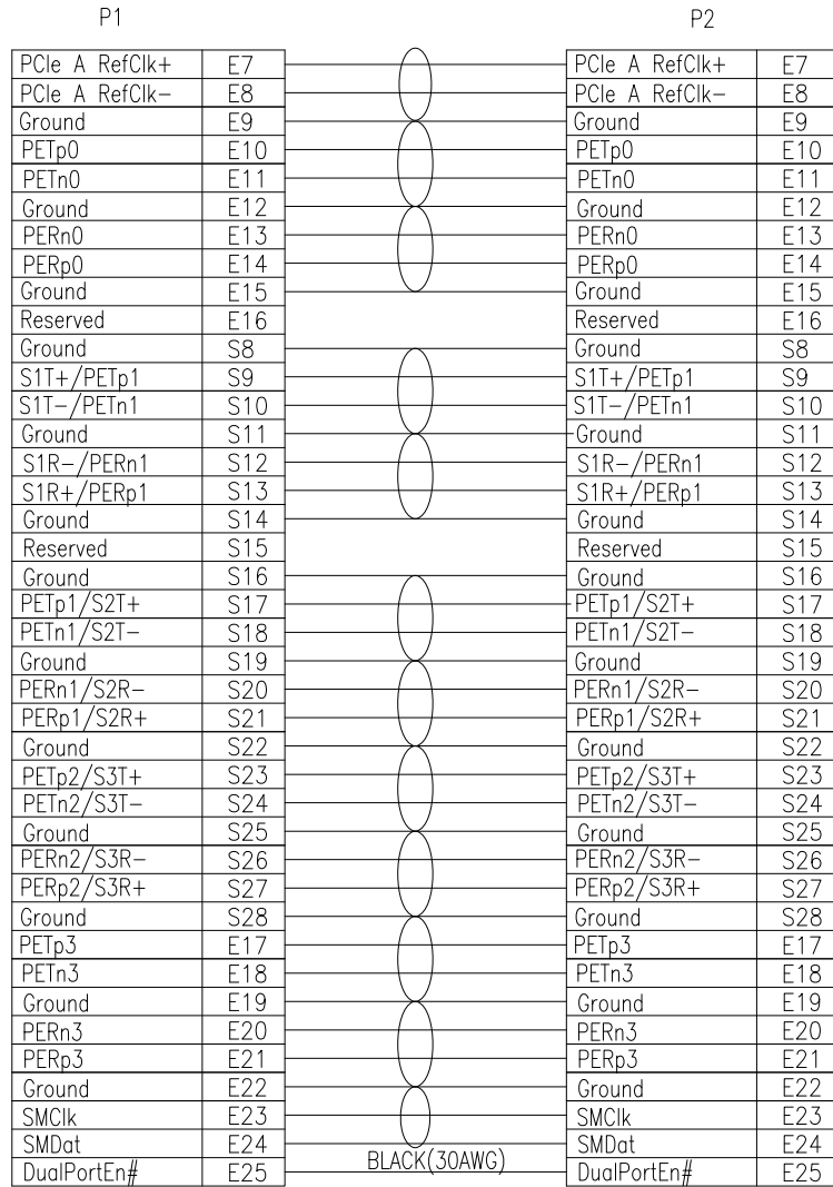
WIRING DIAGRAM
